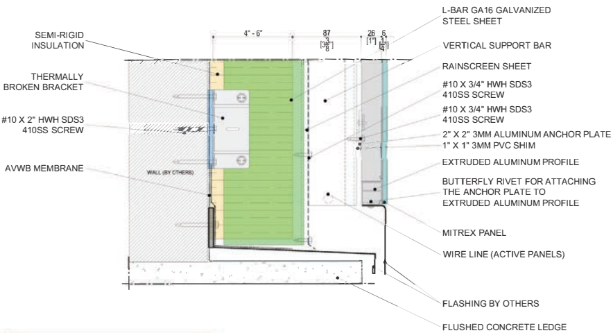
ANCHOR PLATE VERTICAL SUPPORT & POWER BAR
