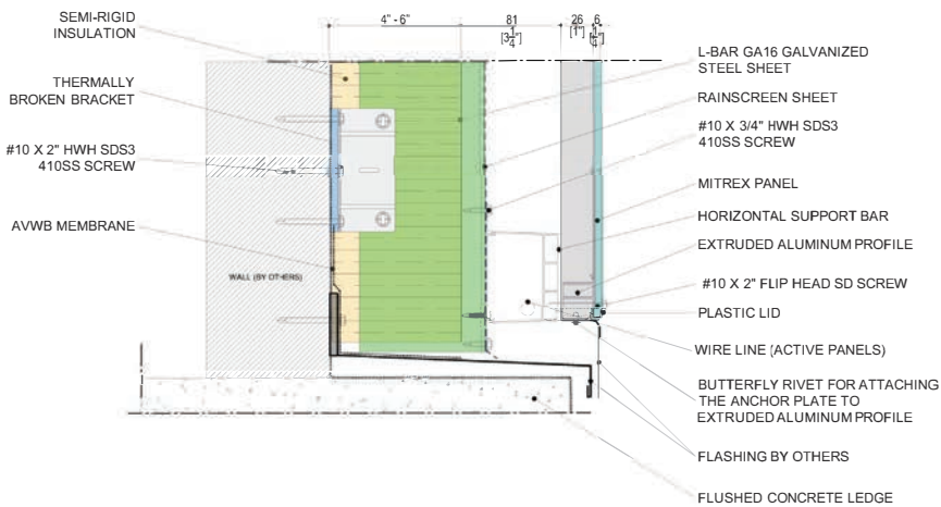
FACE FASTENED HORIZONTAL SUPPORT & POWER BAR
