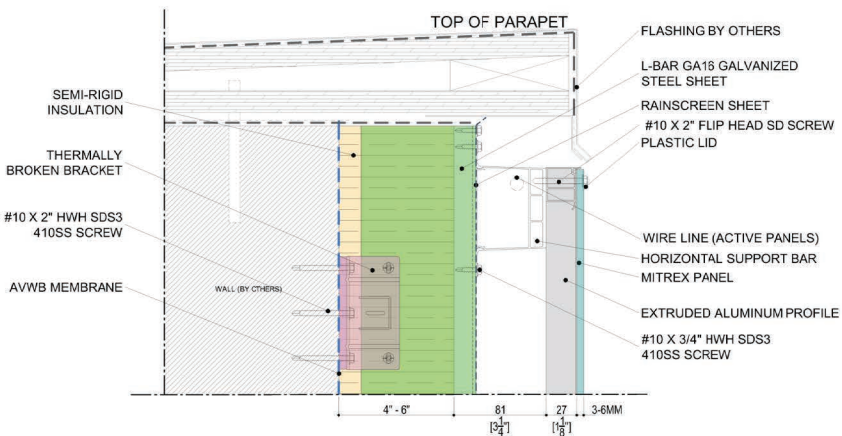
FACE FASTENED HORIZONTAL SUPPORT & POWER BAR
