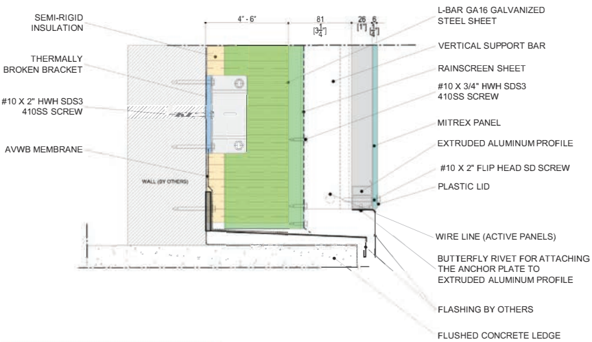
FACE FASTENED VERTICAL SUPPORT & POWER BAR
