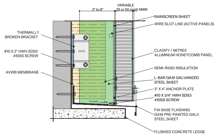
ALUMINUM HONEYCOMB PANEL
