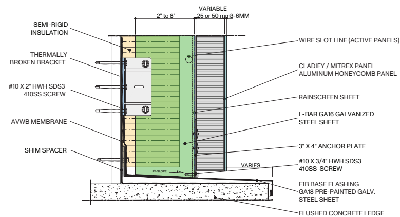
ALUMINUM HONEYCOMB PANEL
