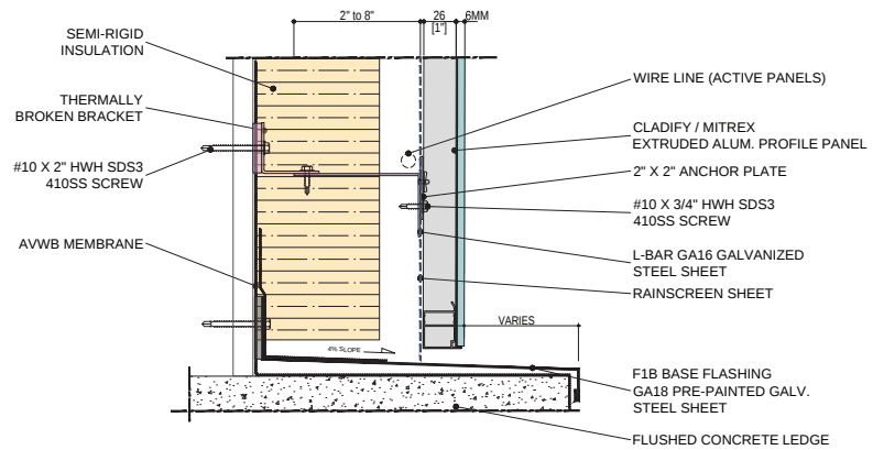
RECESSED PANEL (ANCHOR PLATE - SIDE CONNECTION)
