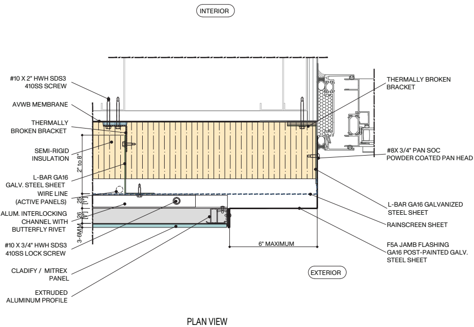
EXTRUDED ALUM. PROFILE PANEL
