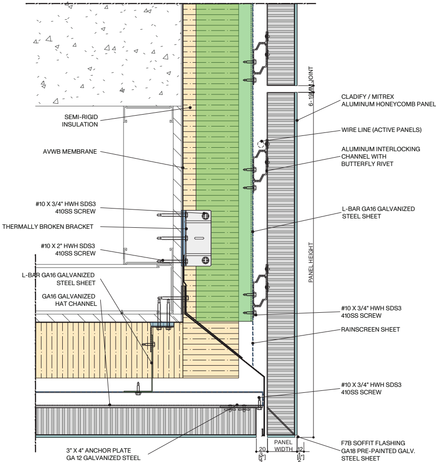
ALUMINUM HONEYCOMB PANEL
