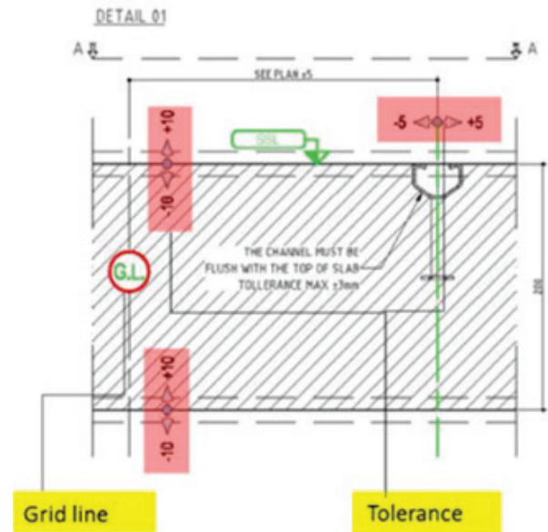
Figure 2: Cast-in channels and structure tolerances.
