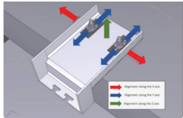
Figure 3: Bracket set
