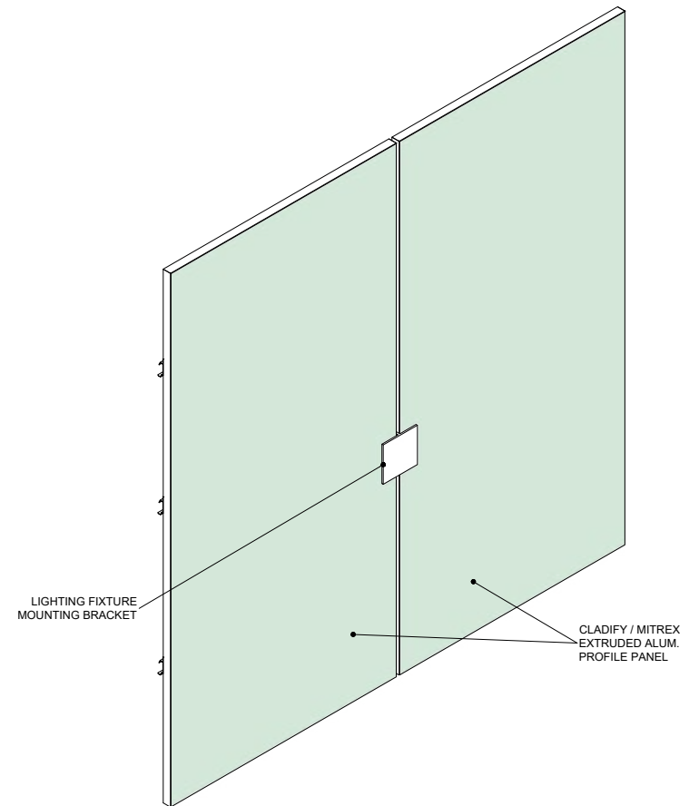
REAR VIEW ISOMETRIC
