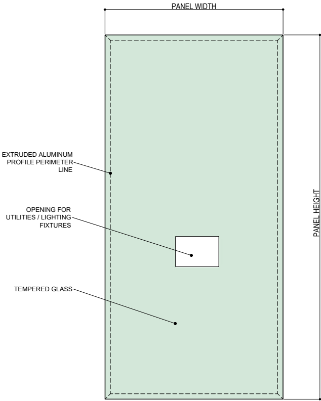
FRONT ELEVATION
