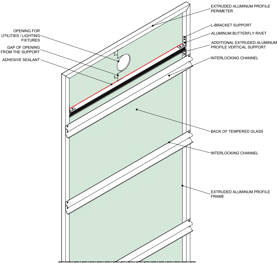
REAR VIEW ISOMETRIC
