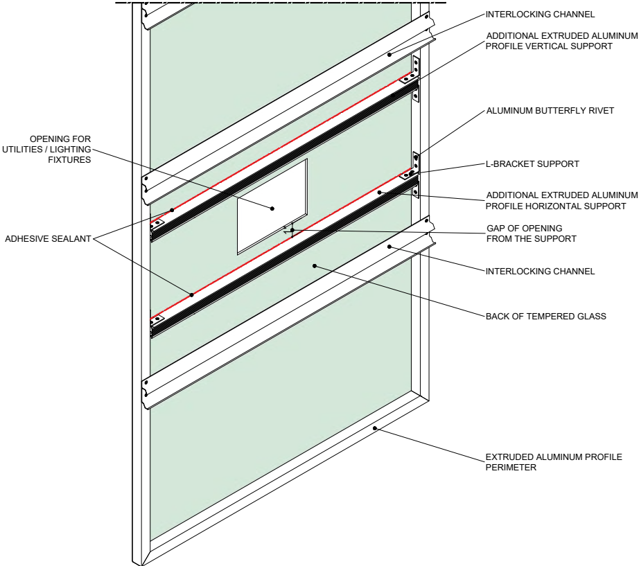
REAR VIEW ISOMETRIC
