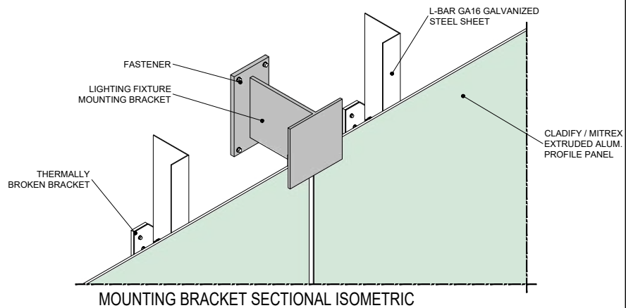
INSERTION OF MOUNTING BRACKET IN BETWEEN 2 PANELS
