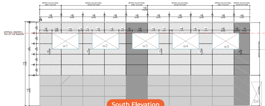
South Elevation
