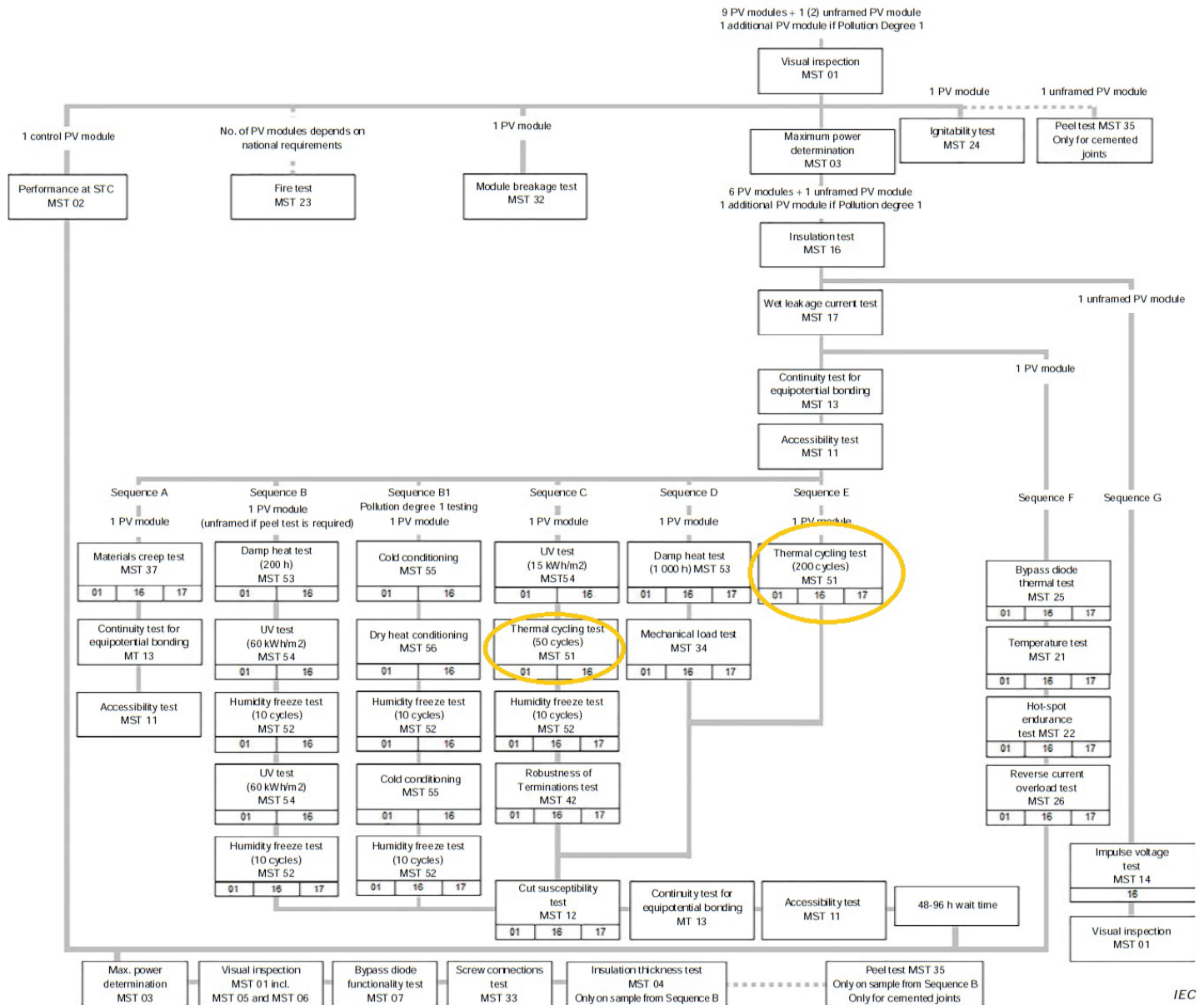
Figure 2 - Test Sequences
