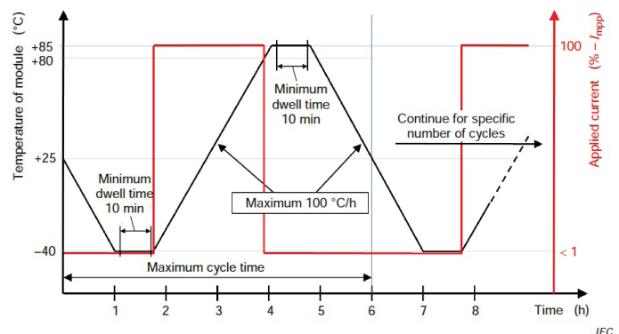
Figure 1: Thermal Cycling Test - Temperature & applied current Profile
