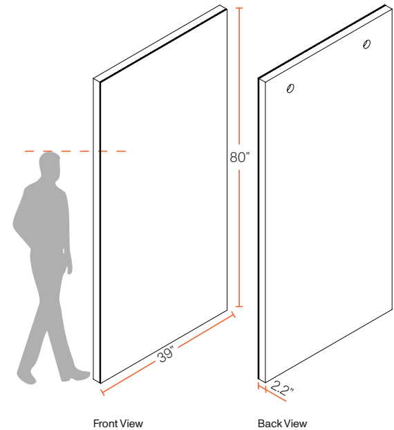
Aluminum Honeycomb
