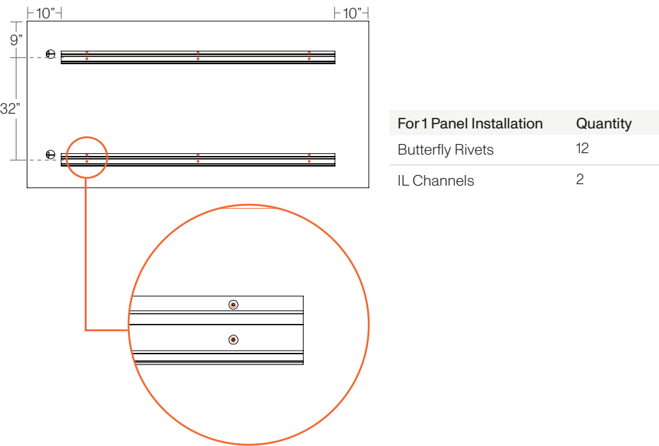
Landscape Installation
