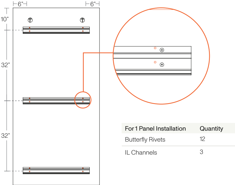
Portrait Installation
