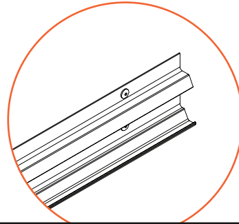
Detail IL channel secured with rivets
