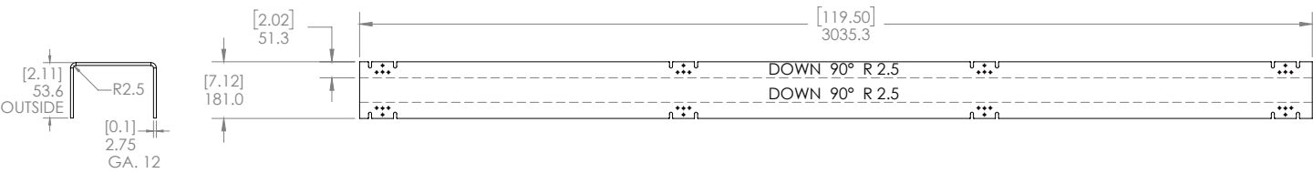
Side View
